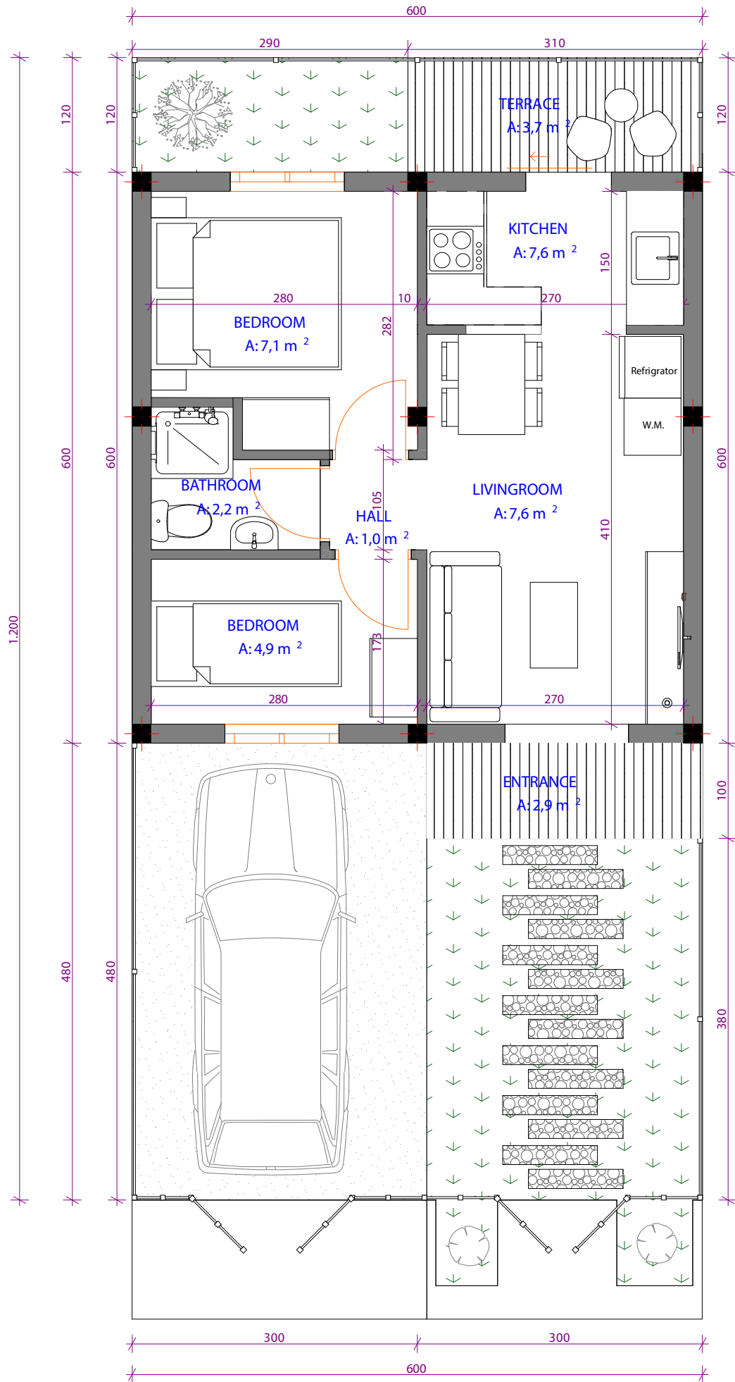
SINGLE STORY HOUSE PLAN 36/72 - (6mx12m)
